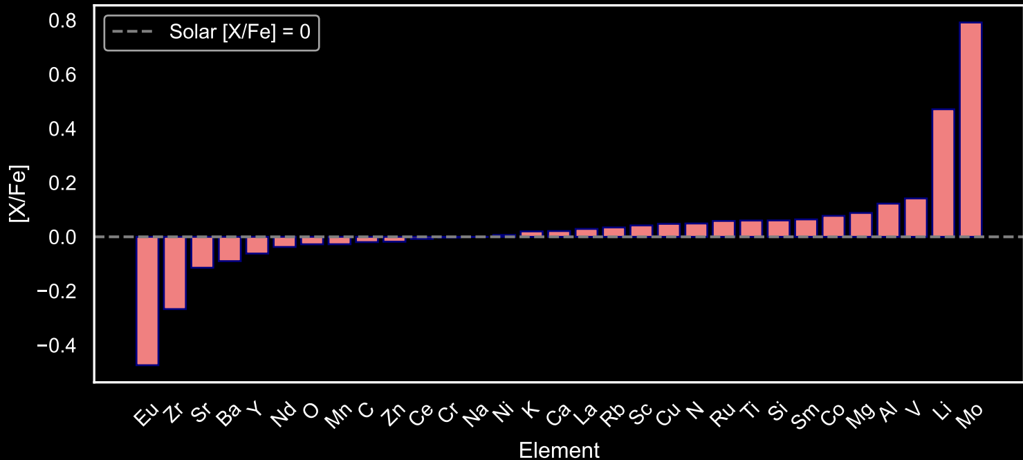
Abundance Pattern for GALAH Main Sequence Stars: Star Field [12] (N=158)
