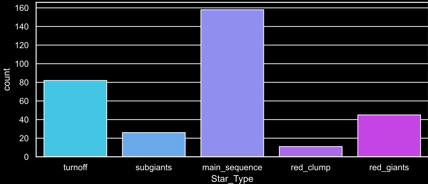
Field [12] Count plot of Star Type
