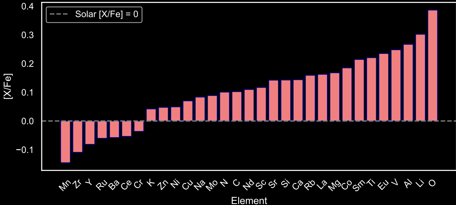
Abundance Pattern for GALAH Red Giants: Star Field [12] (N=56)
