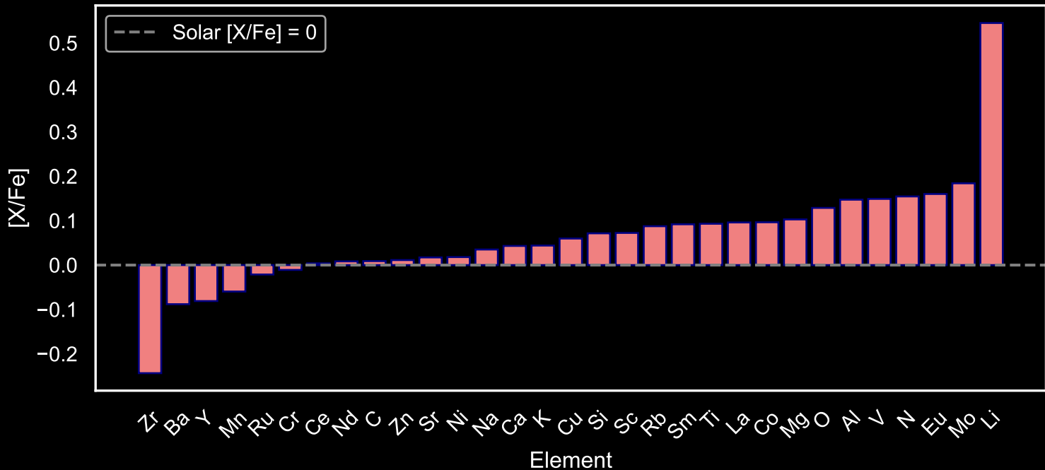
Abundance Pattern for GALAH Star Field [12] (N=322)
